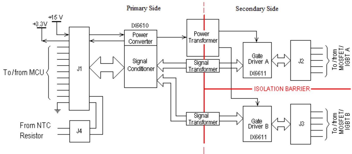
Figure 5. IXIDM1401_O Block Diagram
