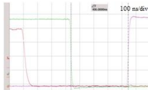
Figure 9 (b). Complementary Signal Dead Time Channel A to Channel B
