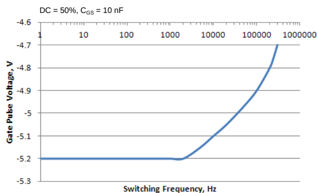
Figure 13. Gate Logic 0 Voltage vs. Switching Frequency
