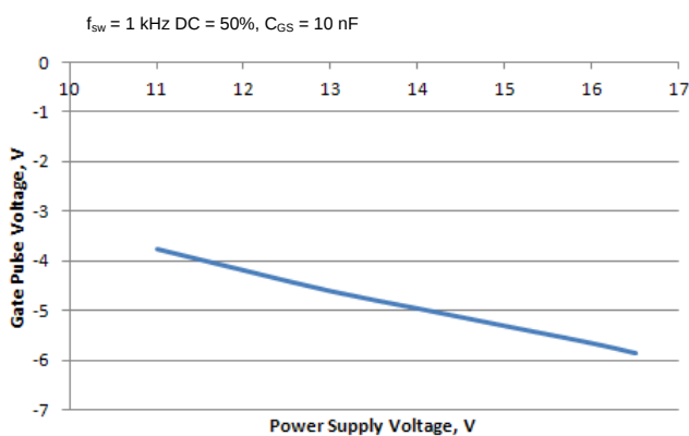
Figure 15. Gate Logic 0 Voltage vs. Power Supply Voltage
